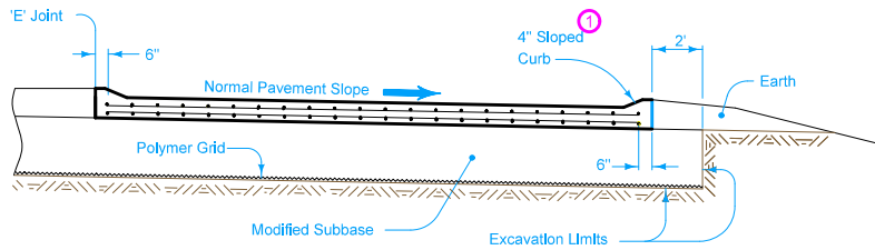
SECTION C-C
