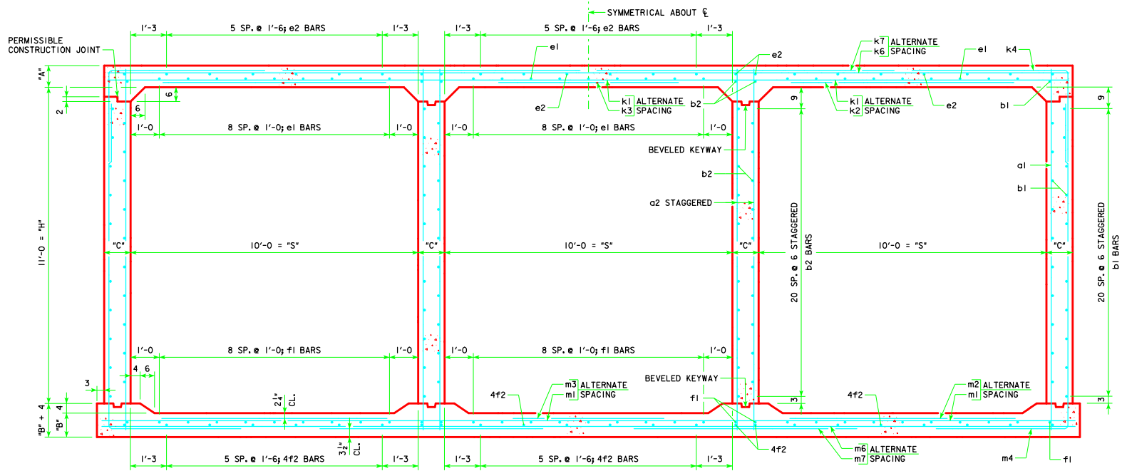
TRIPLE 10 x 11 BARREL SECTION
