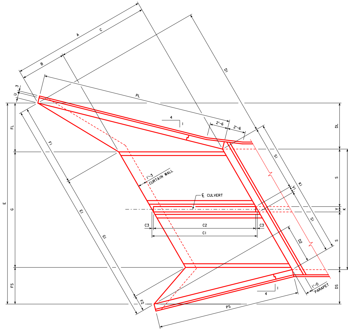
PLAN VIEW
