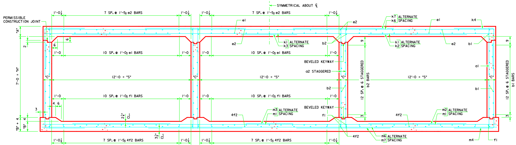
TRIPLE 12 x 7 BARREL SECTION
