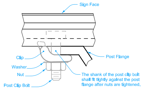
CLIP INSTALLATION
