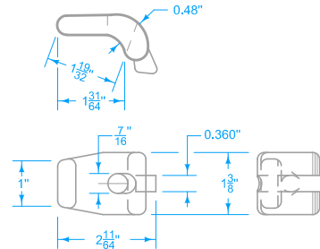
POST CLIP
