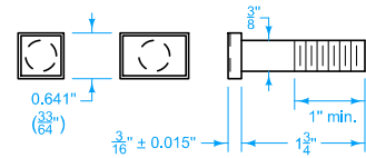
CLIP BOLT (Square or Rectangular Head Optional)
