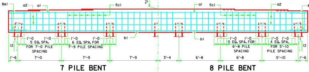
TYPICAL PLAN
