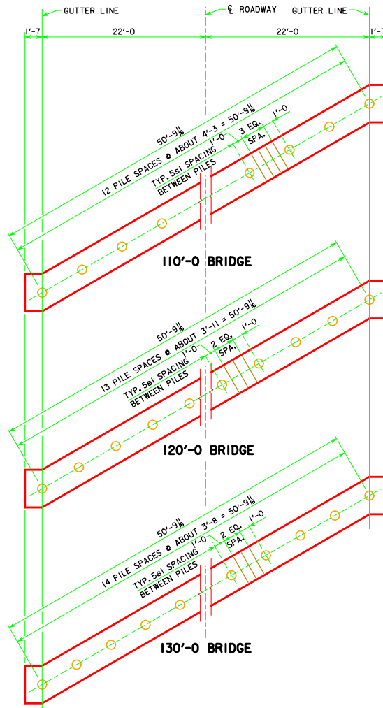
PILE PLAN - 30° SKEW WOOD PILING
