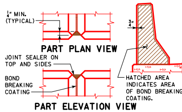
BARRIER RAIL JOINT DETAILS
