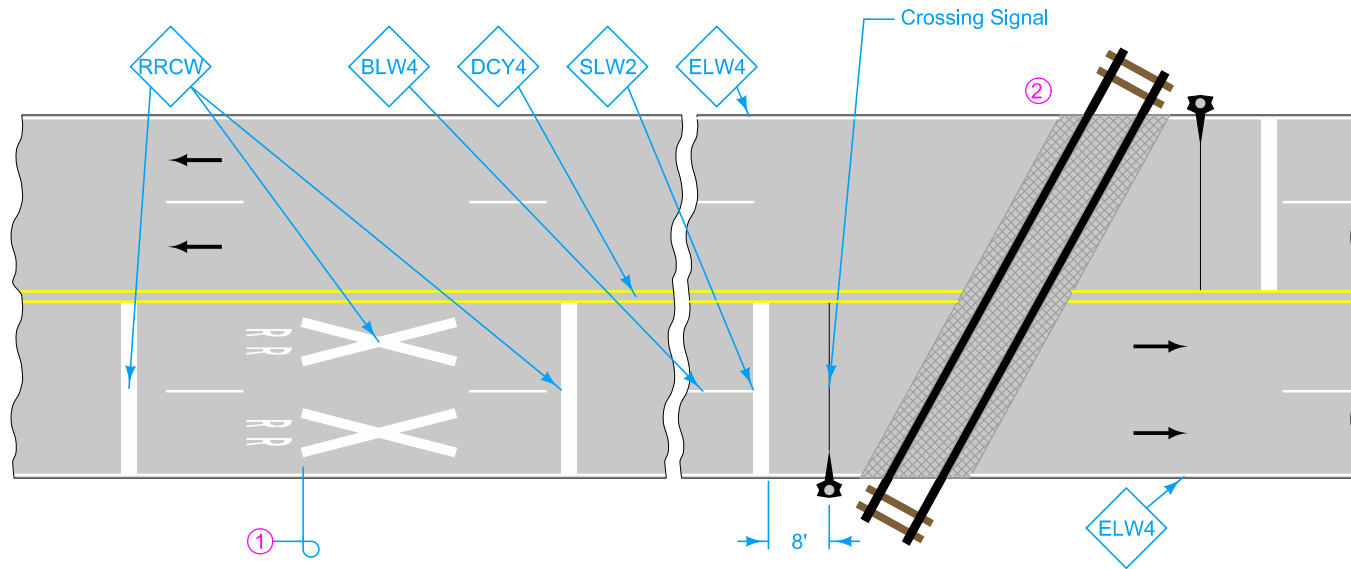
CROSSING WITH CROSSING SIGNAL
