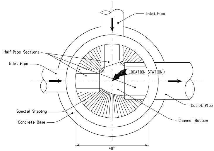
TYPICAL PLAN
