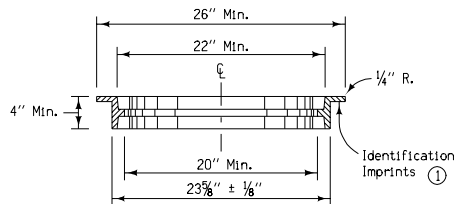
SECTION A-A FRAME DETAILS
