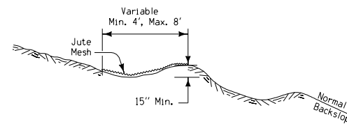
INTERCEPTING DITCH
