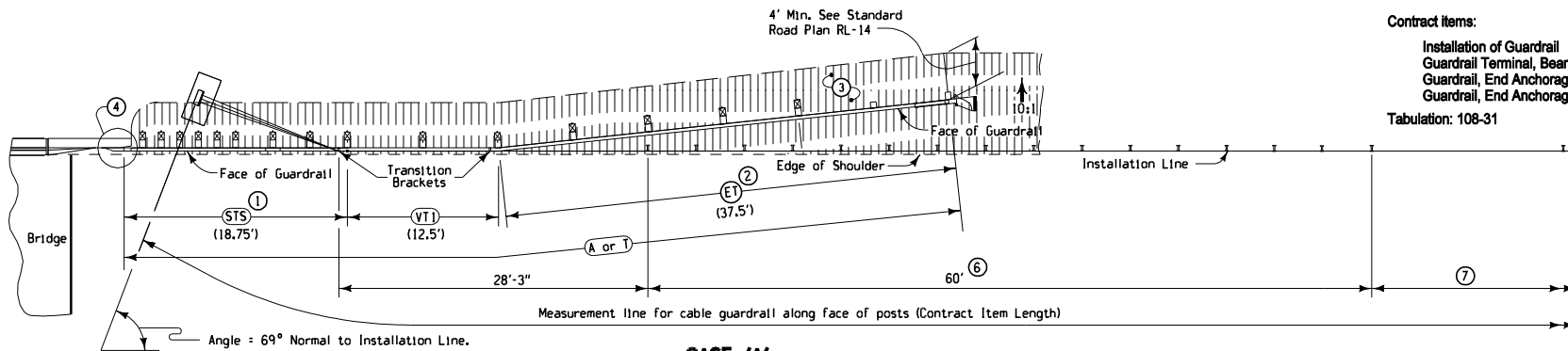
CASE 'A' (Full Shoulder Width Bridge)
