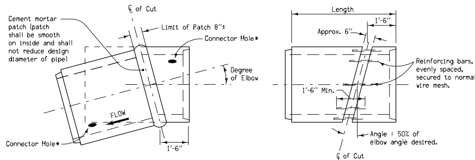
TYPICAL CONCRETE PIPE ELBOW
