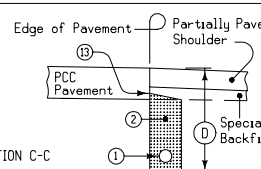
TYPE 7B INSTALLATION SECTION C-C
