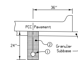
TYPE 12 INSTALLATION SECTION D-D
