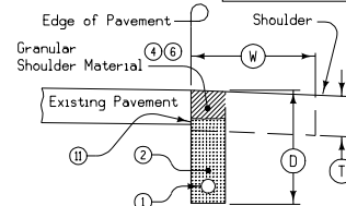
TYPE 10 INSTALLATION SECTION C-C HMA Base Widening
