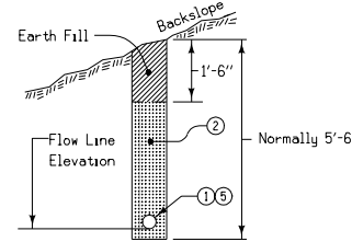
TYPE 11 INSTALLATION SECTION B-B Backslope
