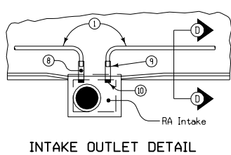
INTAKE OUTLET DETAIL
