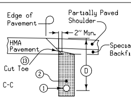
TYPE 8B INSTALLATION SECTION C-C
