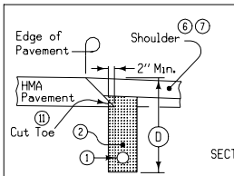
TYPE 8A INSTALLATION SECTION C-C
