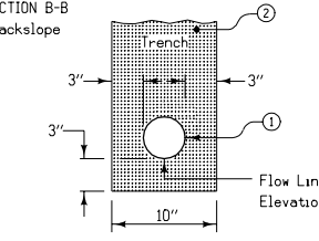
TUBING PLACEMENT DETAIL ALL TYPES
