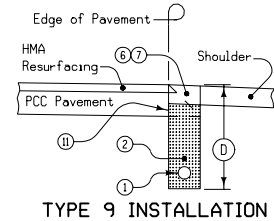
TYPE 9 INSTALLATION SECTION C-C Composite Pavement with Existing Shoulder
