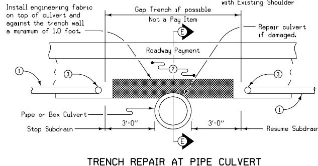
TRENCH REPAIR AT PIPE CULVERT
