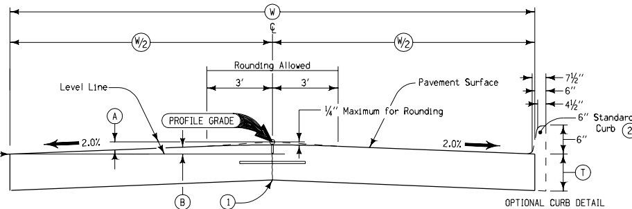
OFFSETS FOR 22', 24', 25' AND 28' PAVEMENT
