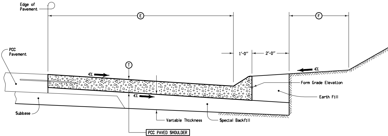
TYPICAL SECTION PCC PAVED SHOULDER
