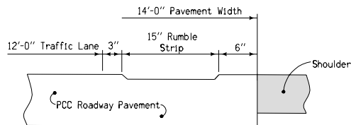
SECTION THROUGH PAVEMENT EDGE
