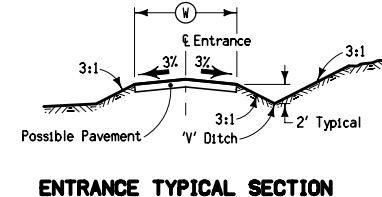
ENTRANCE TYPICAL SECTION
