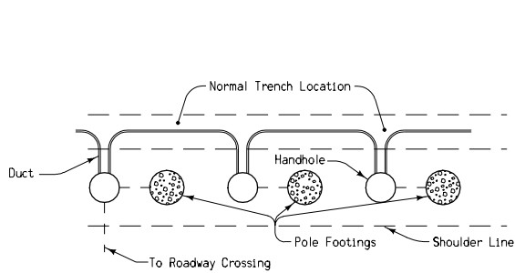
TYPICAL LAYOUTS ① CONNECTIONS TO POLE FOOTINGS
