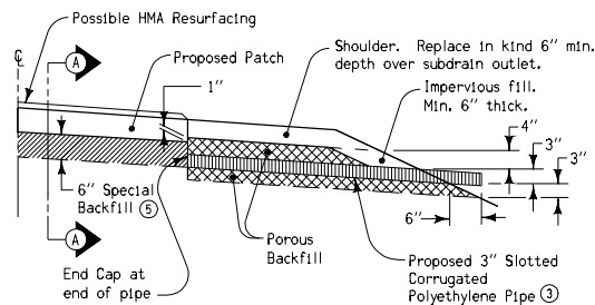
SPECIAL BACKFILL AND SUBRAIN WITHOUT LONGITUDINAL SUBRAIN
