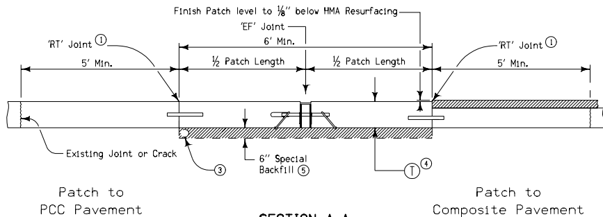
SECTION A-A DOWELED PCC PAVEMENT
