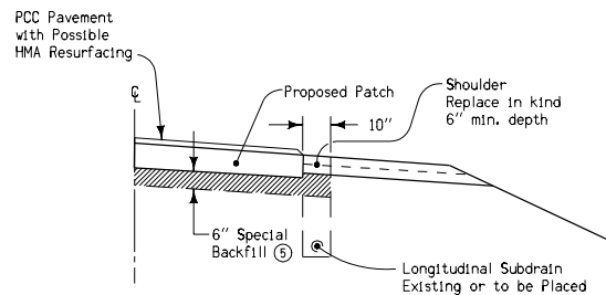
SPECIAL BACKFILL AND SUBRAIN IF LONGITUDINAL SUBRAIN IS PRESENT OR IS TO BE PLACED
