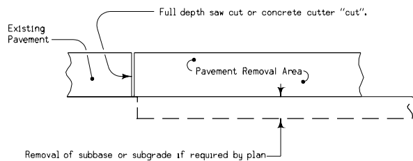
PAVEMENT REMOVAL DETAILS LONGITUDINAL SECTION
