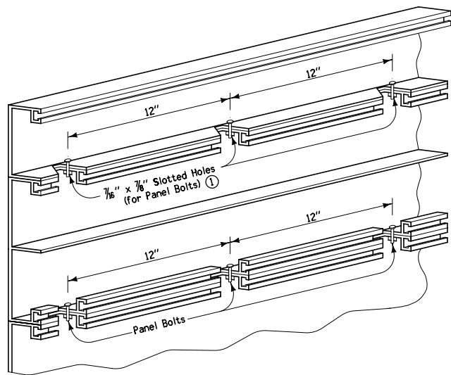
ASSEMBLY DETAIL
