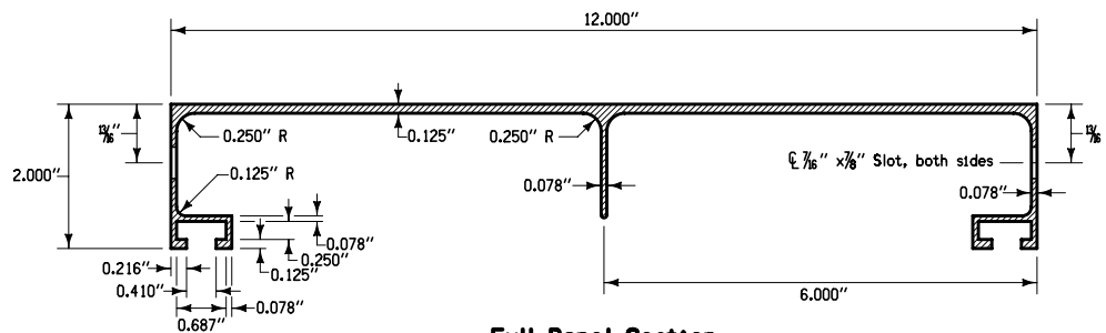
Full Panel Section STANDARD STRUCTURAL SIGN PANELS
