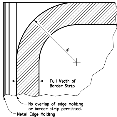
EDGE MOLDING BORDER STRIP DETAIL
