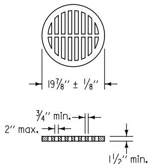
TYPE 4A For Placement on 18" RCP
