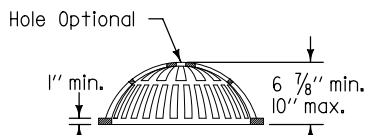
TYPE 3B For Placement on 24" RCP
