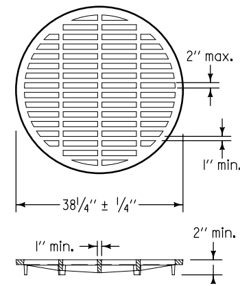
TYPE 4D For Placement on 36" RCP
