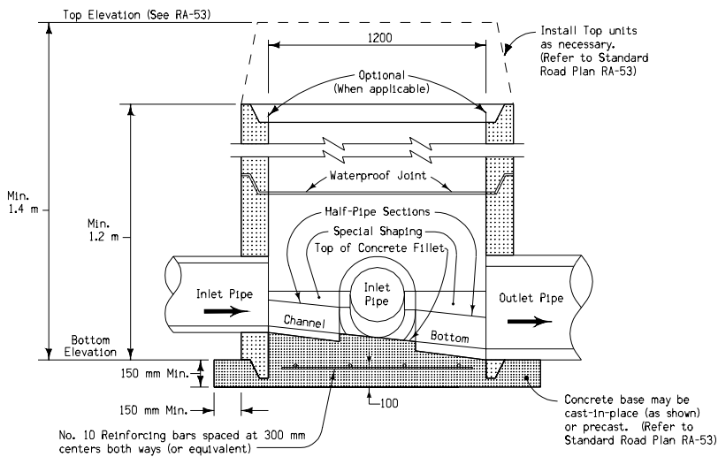
TYPICAL SECTION
