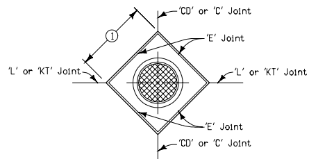
BOX-OUT DETAIL IN PCC PAVEMENT
