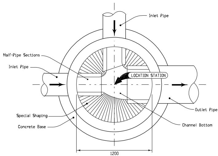
TYPICAL PLAN
