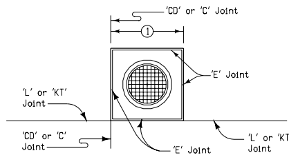
BOX-OUT DETAIL IN PCC PAVEMENT
