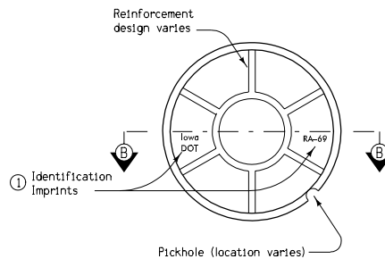
PLAN OF COVER BOTTOM
