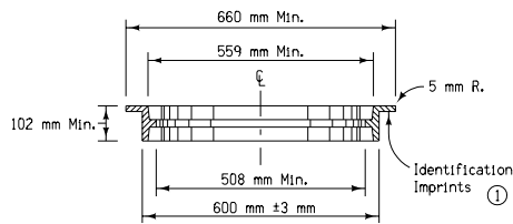
SECTION A-A FRAME DETAILS
