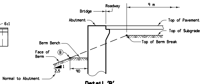
Detail 'B'
