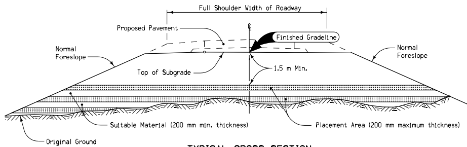
TYPICAL CROSS SECTION TYPE "A" PLACEMENT
