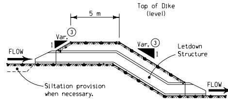
(TYPE F) TYPICAL SECTION C-C
