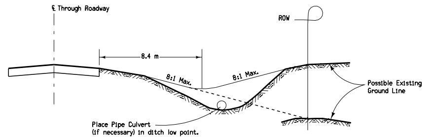
SECTION B-B
