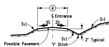
ENTRANCE TYPICAL SECTION
