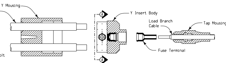
DETAILS OF TYPE Y-1 CONNECTOR DISASSEMBLED CONNECTOR
