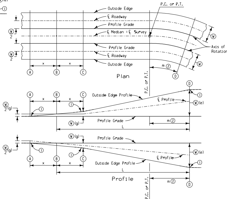
TRANSITION DETAILS WHEN SPIRAL IS NOT USED
