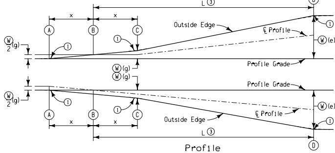
TRANSITION DETAILS WHEN SPIRAL IS USED
