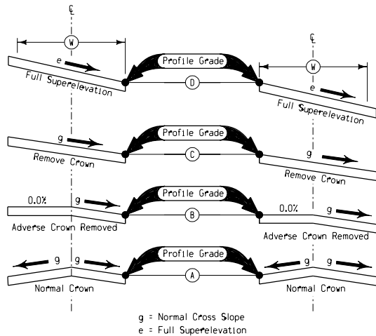
AXIS OF ROTATION AT ADJACENT PAVEMENT EDGES
