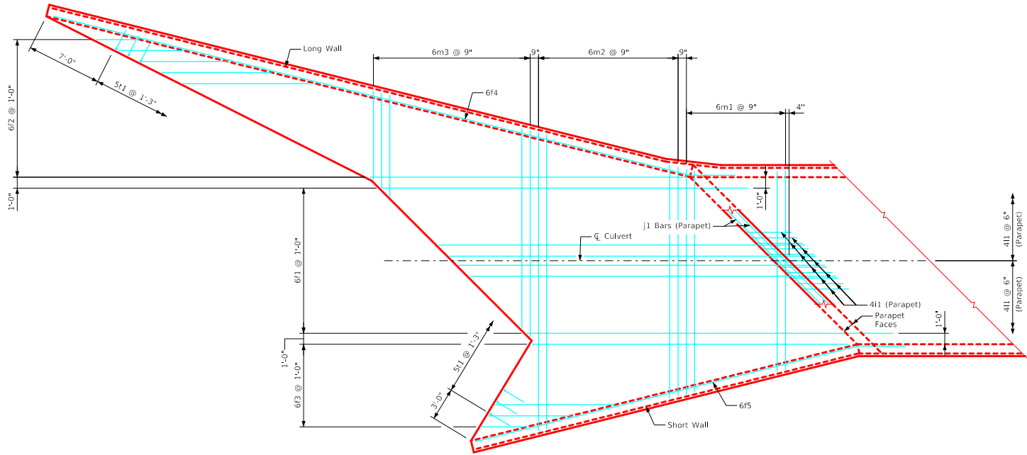
Plan View - Top of Apron Reinforcing
