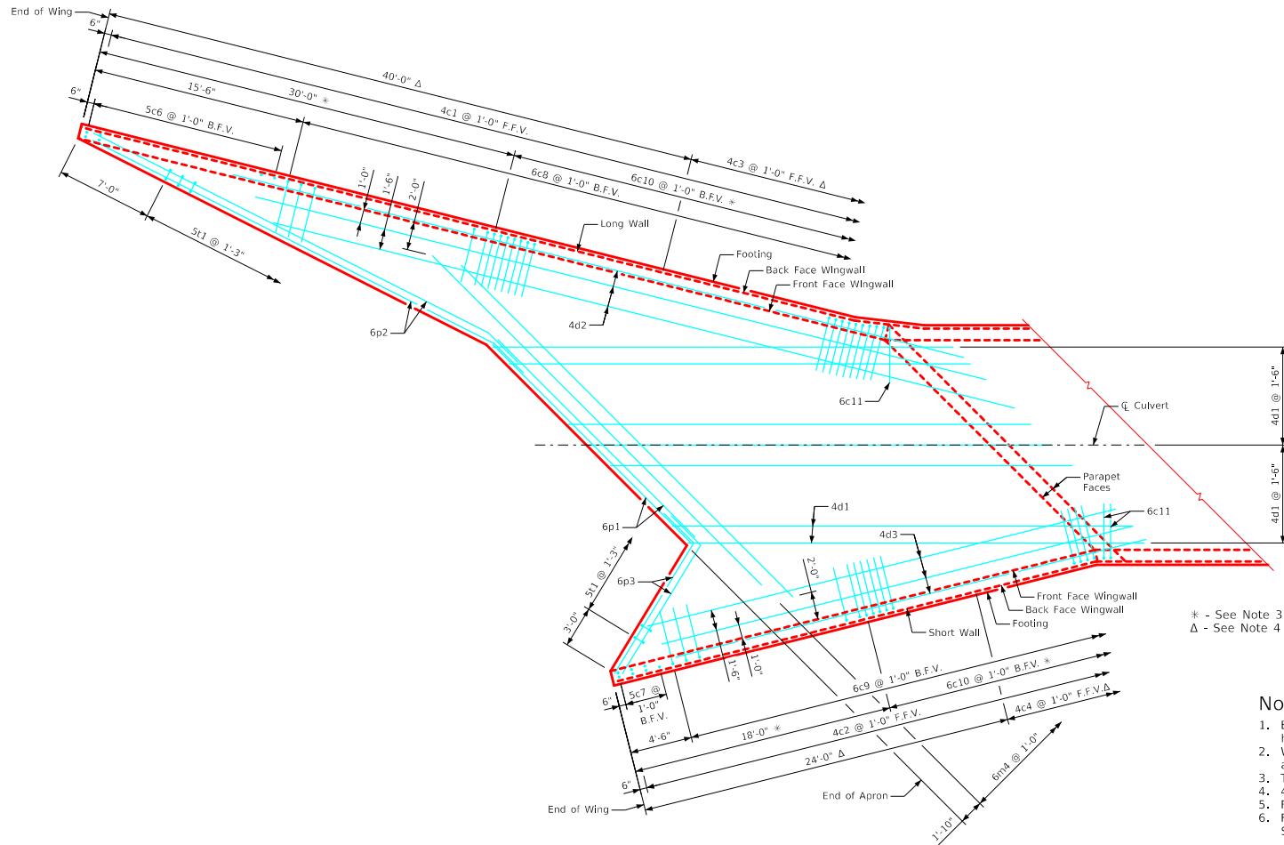
Plan View - Bottom of Apron Reinforcing Bars
