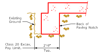
Paving Notch Class 20 Excavation
