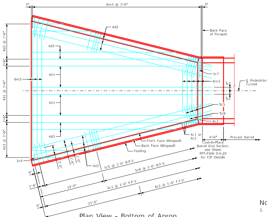
Plan View - Bottom of Apron Reinforcing Bars (Paving Notch Not Shown for Clarity)
