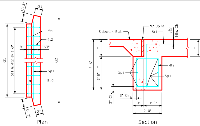
Paving Notch Details
