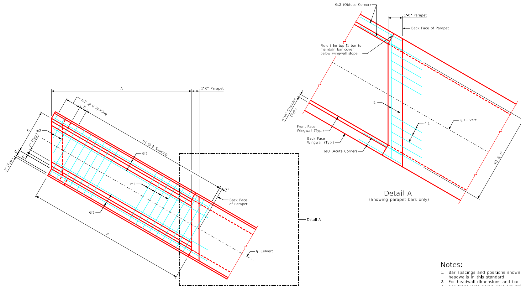
Plan View - Top Apron Reinforcing (Wall Reinforcing not shown for clarity)
