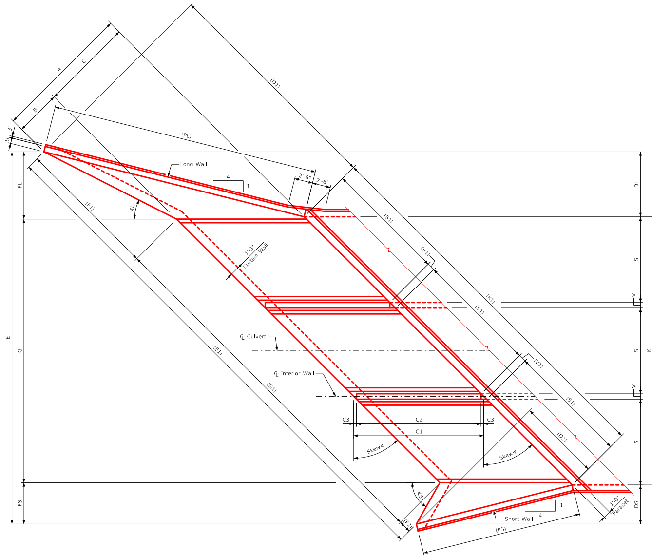
Plan View
