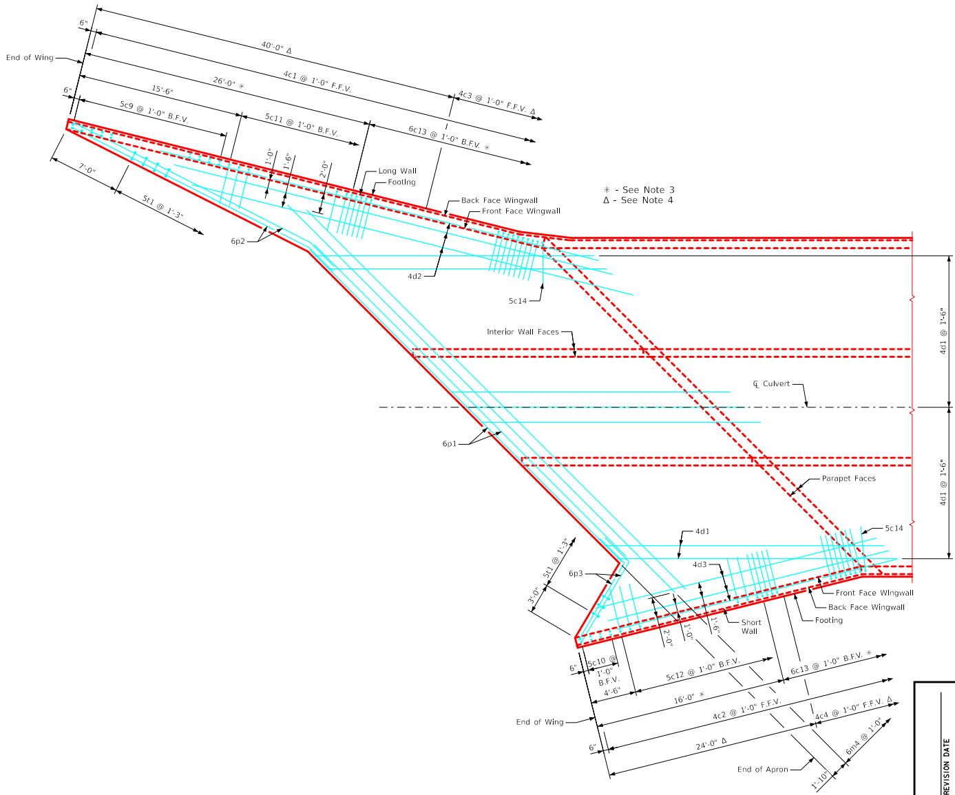
Plan View - Bottom of Apron Reinforcing
