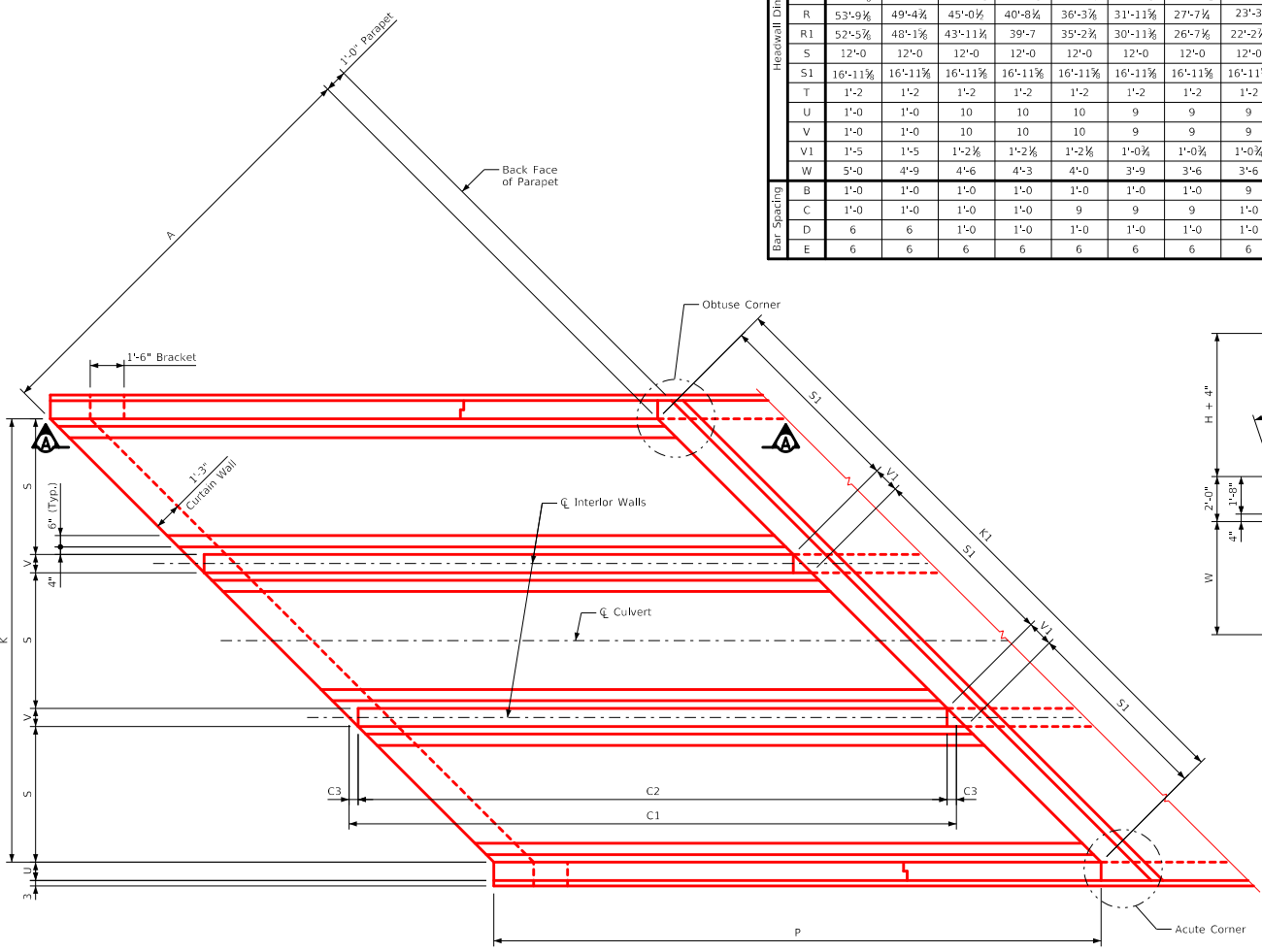
Plan View
