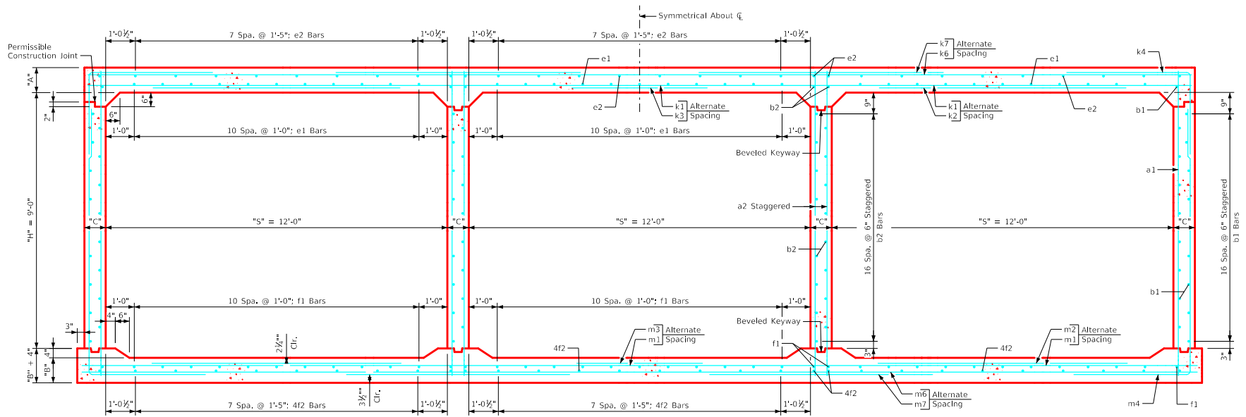
Triple 12' x 9' Barrel Section
