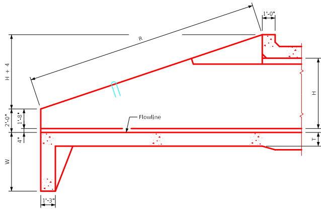
Elevation Section A-A
