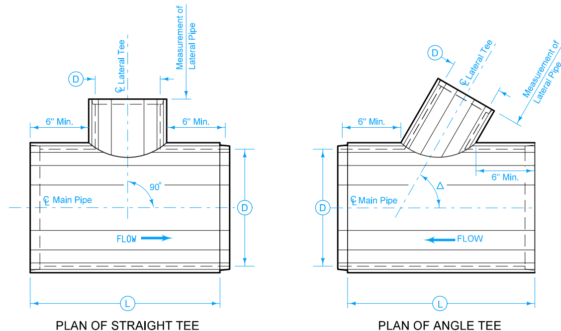
PLAN OF STRAIGHT TEE
