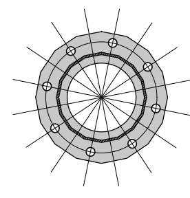
EIGHT ANCHOR BOLT PATTERN FOR HEXADECAGON (16) TOWER SECTION
