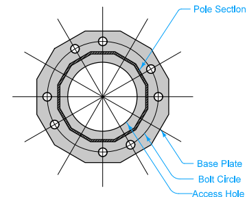
EIGHT ANCHOR BOLT PATTERN FOR DODECAGON (12) TOWER SECTION
