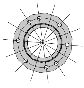
EIGHT ANCHOR BOLT PATTERN FOR TETRADECAGON (14) TOWER SECTION
