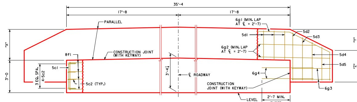
REAR ELEVATION AT ABUTMENT
