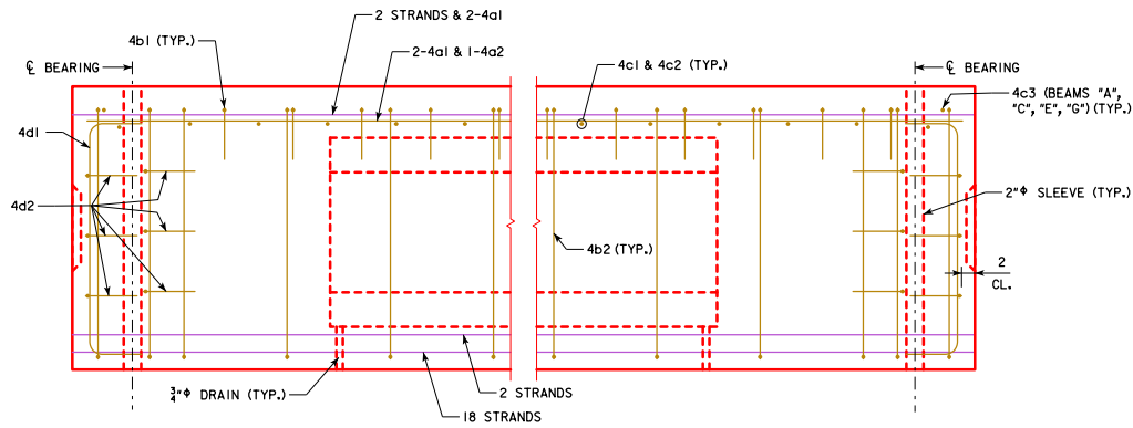
ELEVATION (KEYWAY NOT SHOWN FOR CLARITY)
