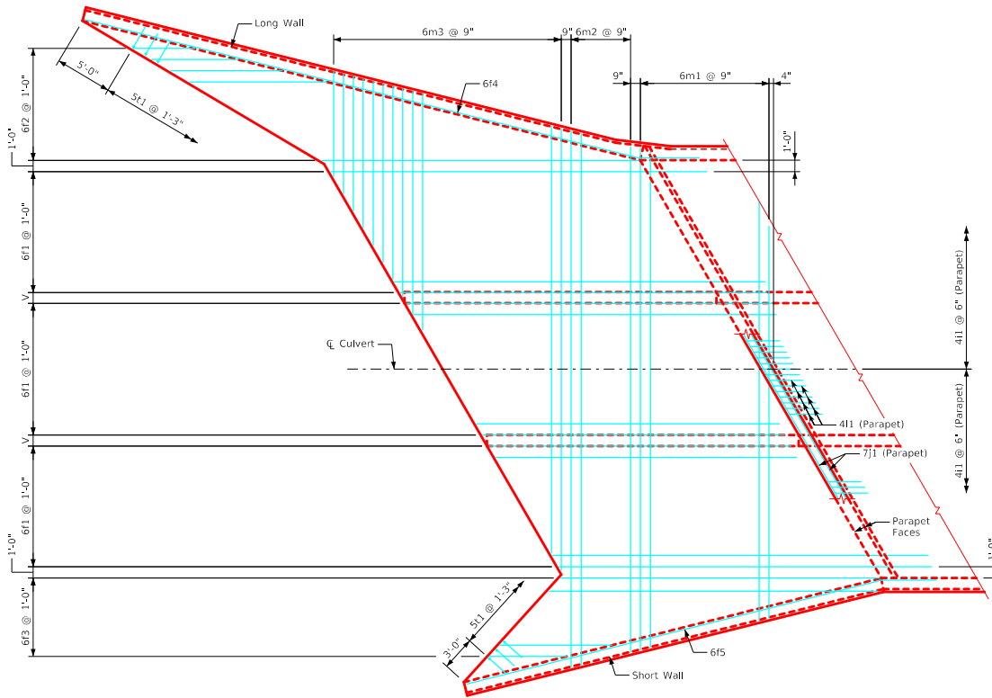
Plan View - Top of Apron Reinforcing
