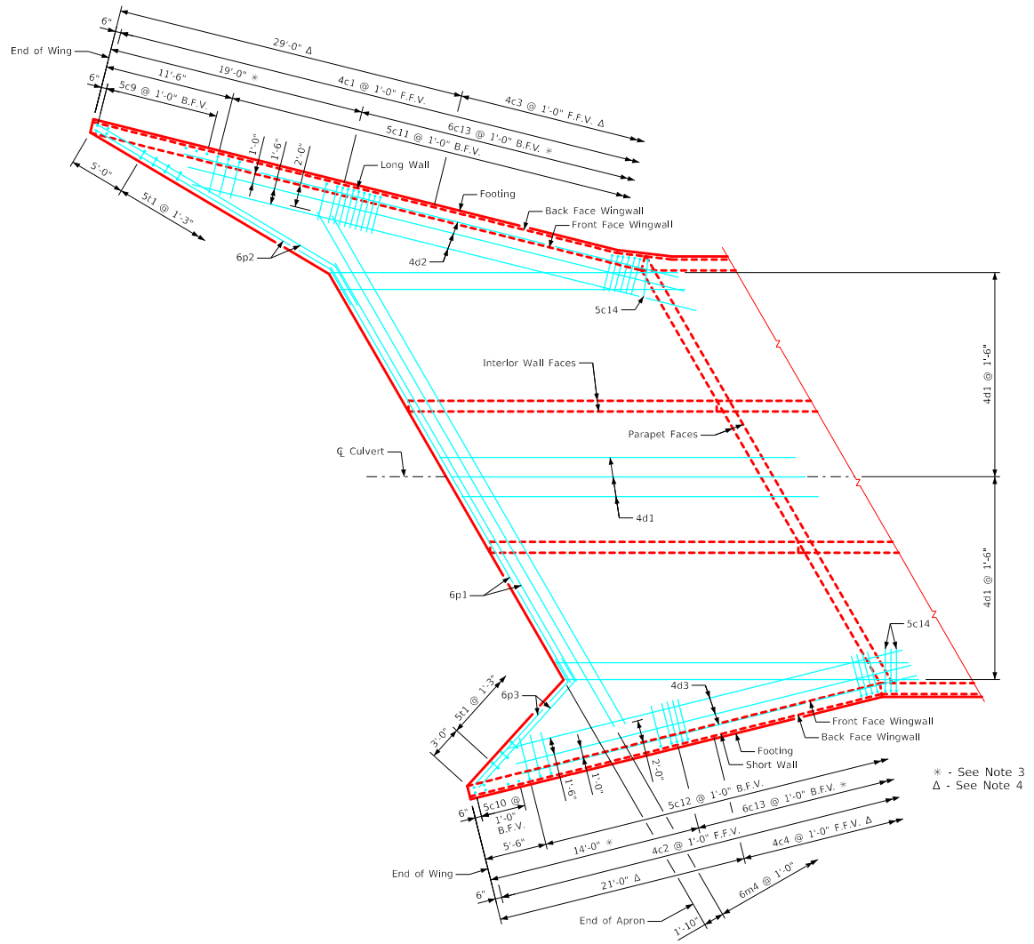
Plan View - Bottom of Apron Reinforcing
