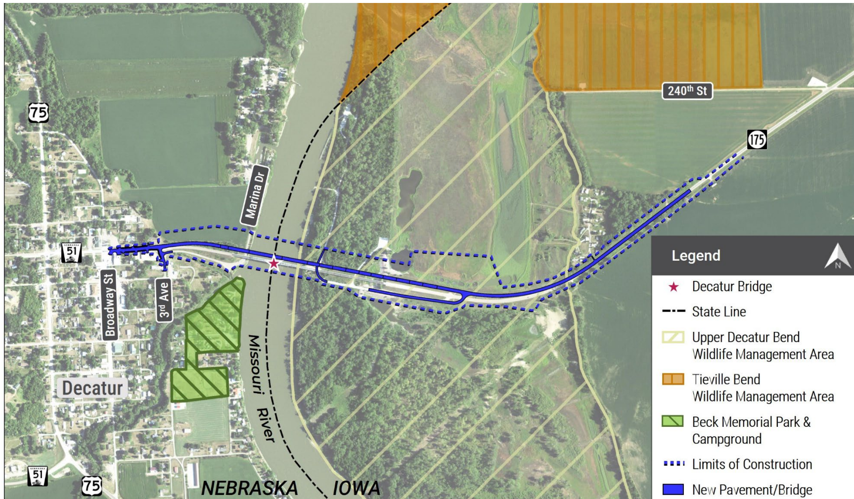
Figure 2-2. Preferred Alternative – Build a New Bridge North of and Parallel to the Existing Decatur Bridge
