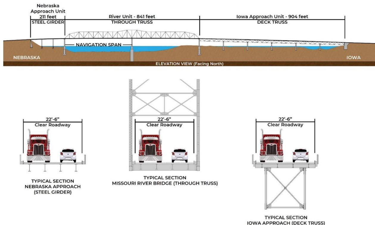
Figure 1-2. Components of the Decatur Bridge
