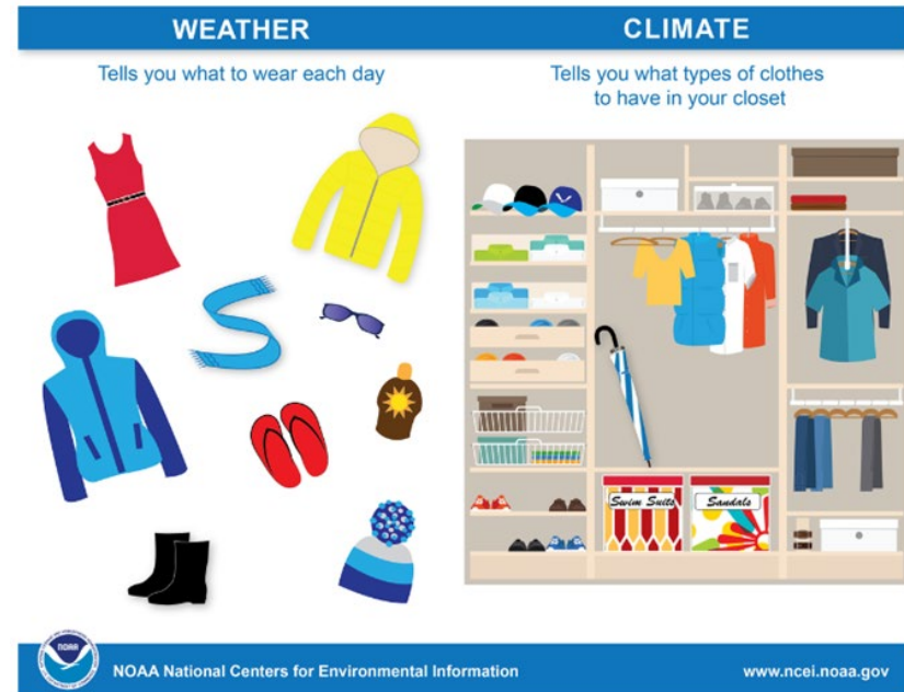
Figure 2.3: Weather vs. climate
